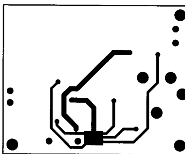
Figure 46. Recommended MM PC Board Layout: Bottom-Side Layout
