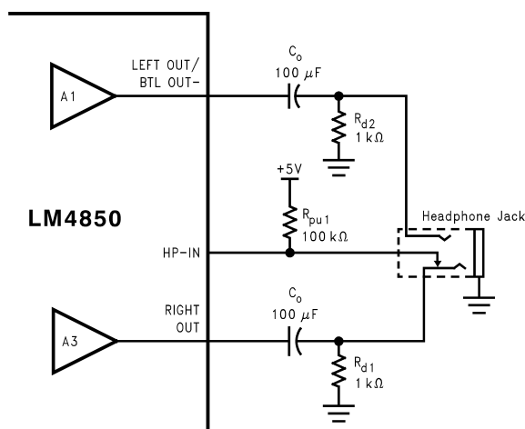
Figure 40. Headphone Control Circuit
