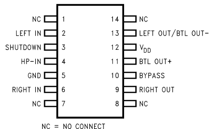
Figure 3. Top View 14 Lead TSSOP See Package Number PW
